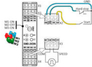
DC brush motor speed control using external PWM signal. Connection diagram
