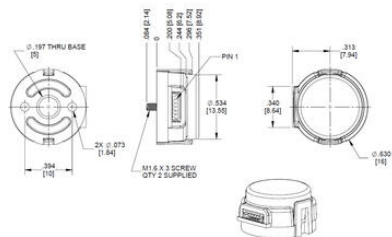
E16 Micro Optical Kit Encoder
